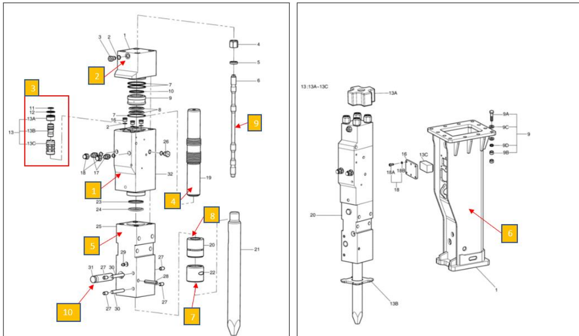
Figure 1.- Breaker Parts
